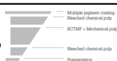
Board structure
